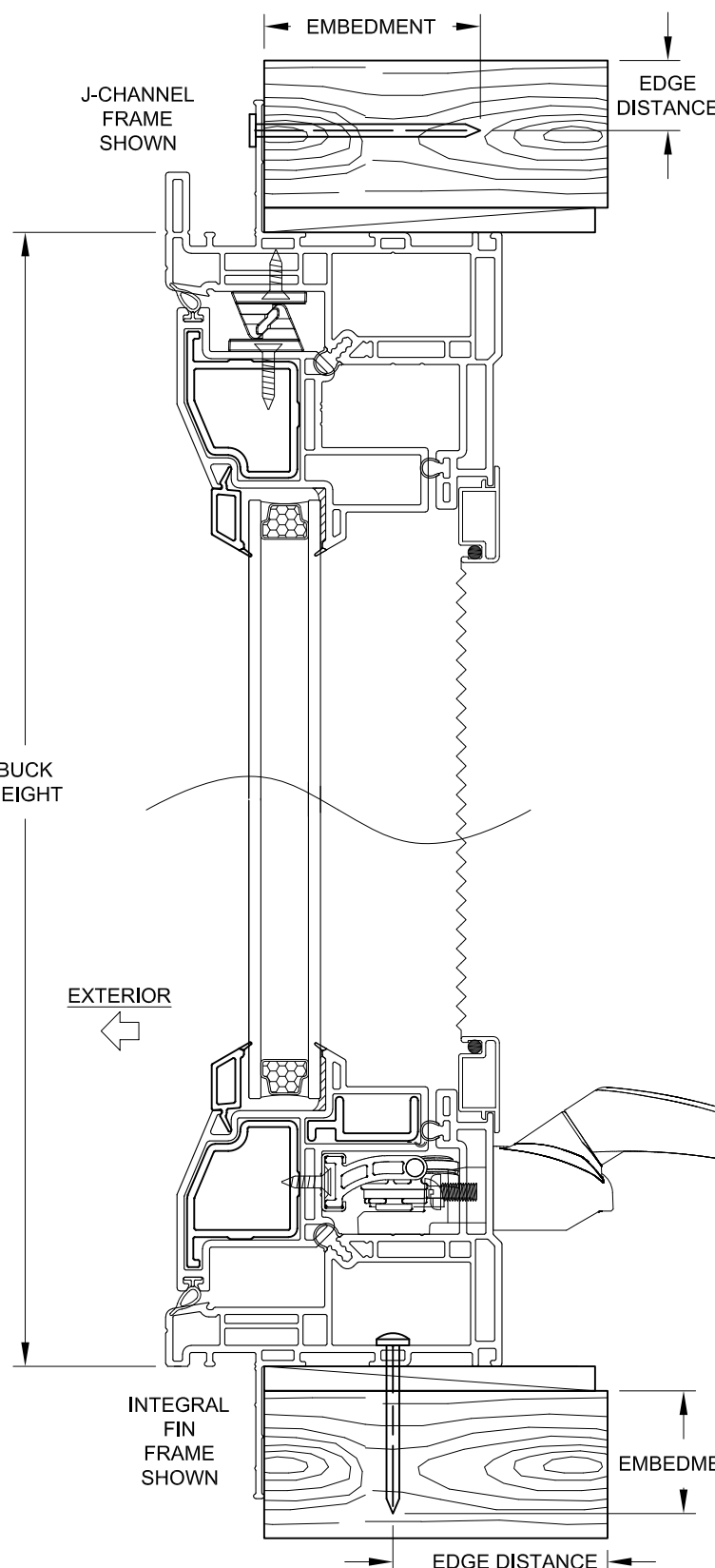
VERTICAL SECTION D-D
