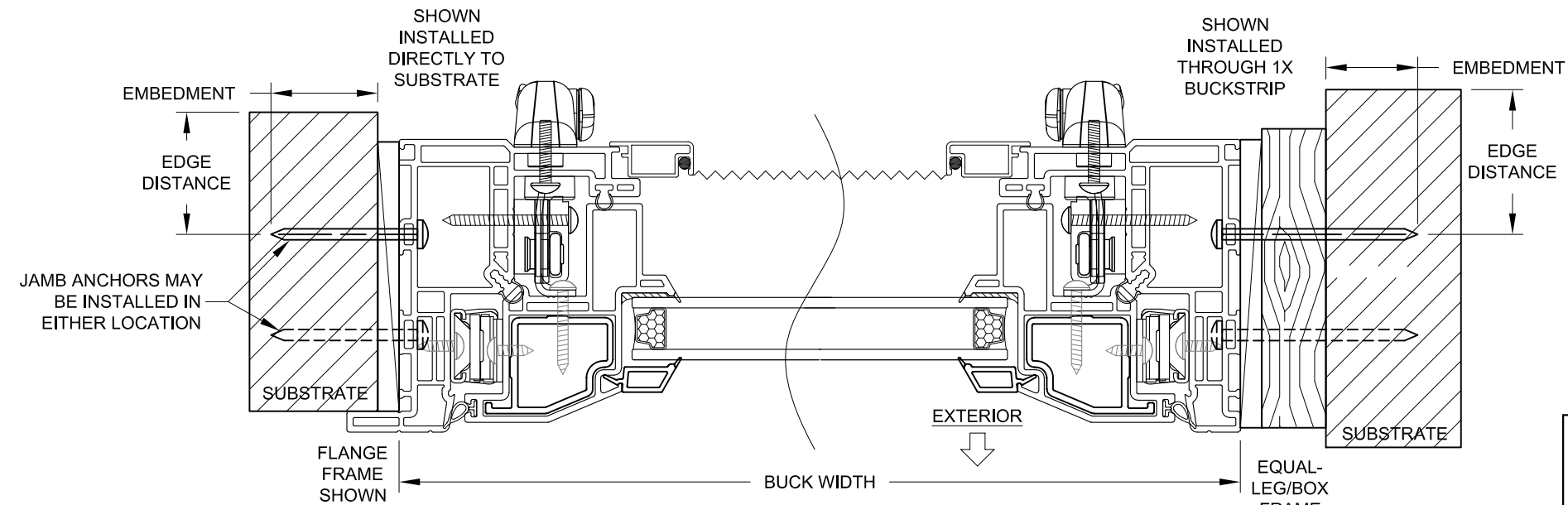
HORIZONTAL SECTION A-A
